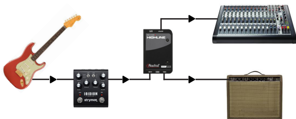
Adding an amplifier to the Thru output
