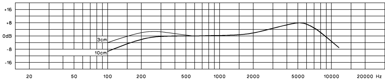
Frequency response curve \pm 2.5 dB 0 dB = 1.3 mV / Pa
