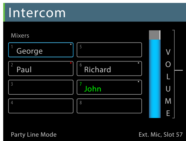
Intercom info is displayed when you hold the Intercom button down. George (on port #1) is an active Speaker as seen from John's A640
